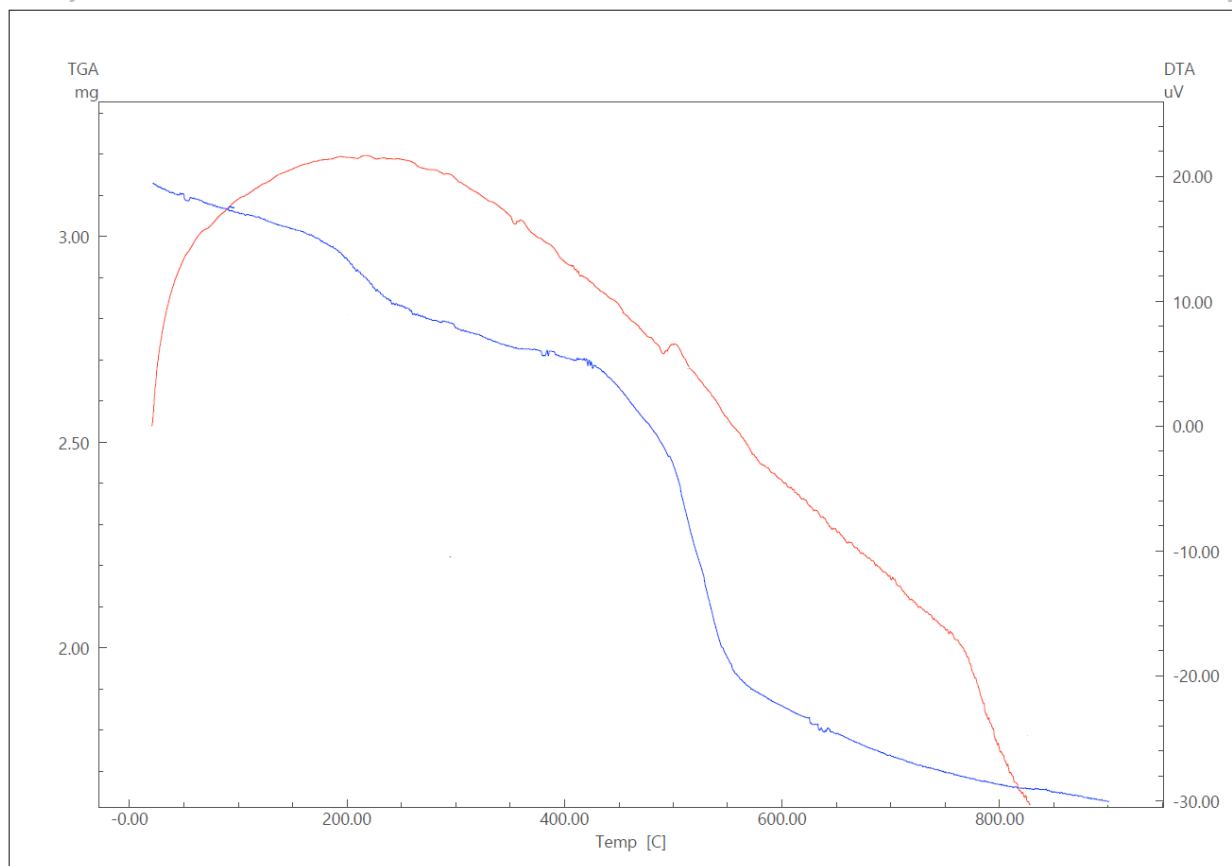
5-rasm. Kraxmal karbamat-epixlorgidrin asosidagi KrK-EXG (1:3) sorbentining termik barqarorligini tavsiflovchi TGA va DTA termogrammalari.
