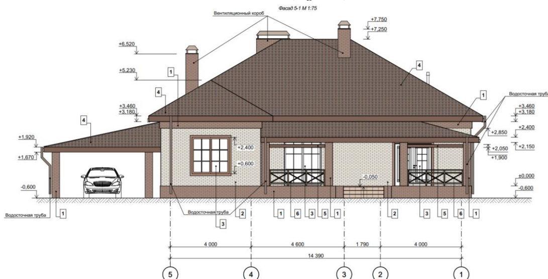
1 - picture. Modern house project
