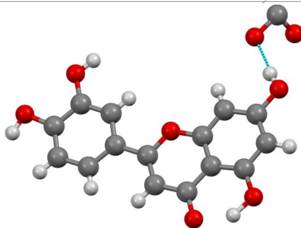
1-rasm. 2-(3,4-dihydroxyphenyl)-5,7-dihydroxy-4H-chromen-4-one+CO 2
