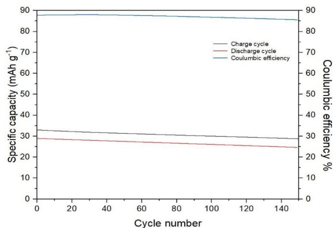
Fig.1. Electrochemical stability test of graphite cathode
