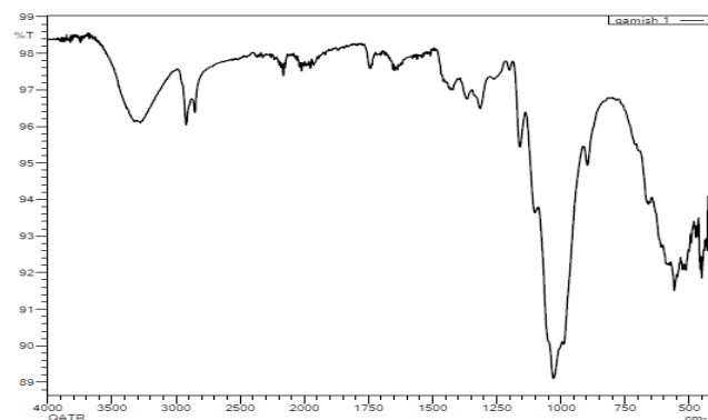
2-rasm. Qamish poyasining IQ spektri
