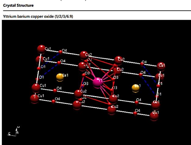
3-rasm. YBCO-(123) kristall panjarasining RST da ko'rinishi
