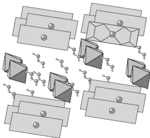
1-rasm. [M(H_2O)_6][PdOx_2] \cdot 4H_2Ox ning kristall tuzilishi ( M = Co, Ni ). [M(H_2O)_6]^{2+} oktaedr bilan, [PdOx_2]^{2-} to'rtburchaklar bilan belgilanadi
