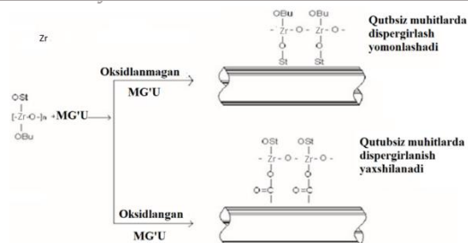
Figure-4. Scheme of functionalization of MPCs with organozirconates
