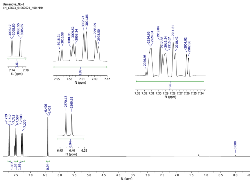
1-rasm. Kumarin 1 H-YaMR spektri
