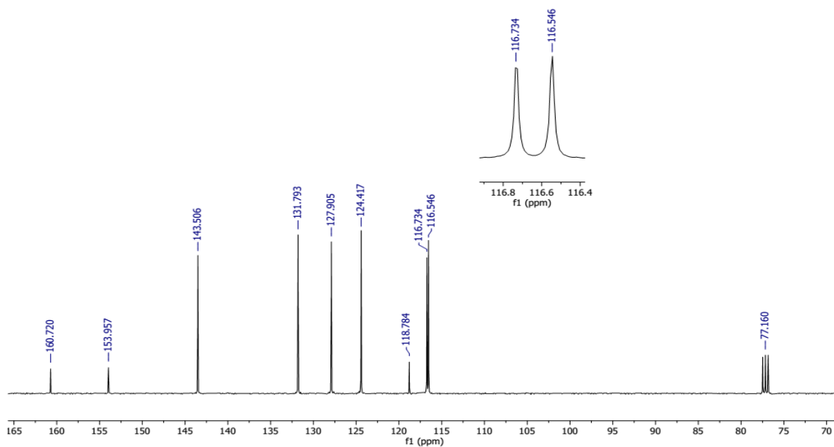
2-rasm. Kumarin 13 C-YaMR spektri
