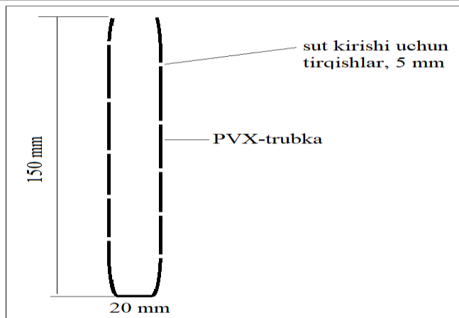
1-rasm. Magnetitli sorbent solinadigan PVX-truba sxemasi
