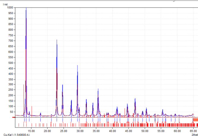
1-rasm. Boshlang'ich opoka minerali rentgenofazaviy tahlili
