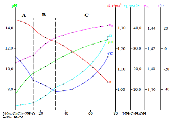
Fig. 3. Component dependence diagram of changes in pH value, density ( d ), viscosity ( \eta ), refractive index ( n_D ) and crystallization temperature ( t^\circ\text{C} ) of [40 % \text{CaCl}_2\cdot 2\text{H}_2\text{O} + 60 % \text{H}_2\text{O} ] – \text{NH}_2\text{C}_2\text{H}_4\text{OH} system solutions.
