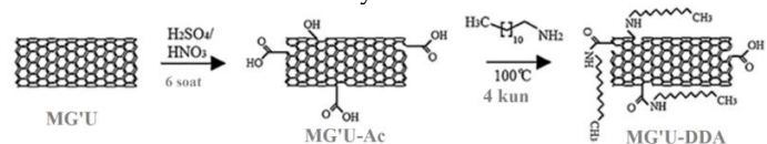
Figure-3. Scheme of functionalization of MPCs with dodecylamine
