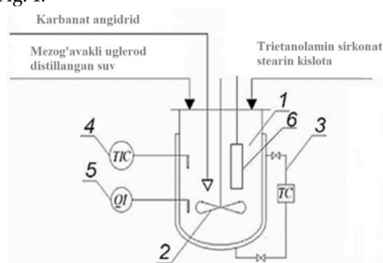
Figure-1. Scheme of a laboratory device for the functionalization of MPCs:
