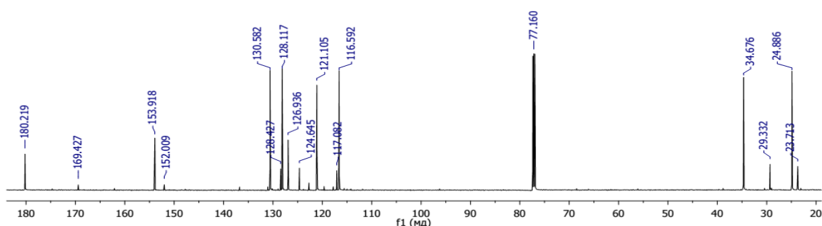
4-rasm. Digidrokumarin 13 C YaMR spektri
