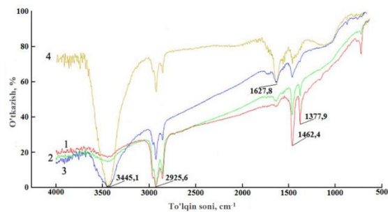
Figure-7. IR spectra of MPC: original (1) and oxidized with concentrated nitric acid for 2 (2); 5 (3) and 10 (4) hours
