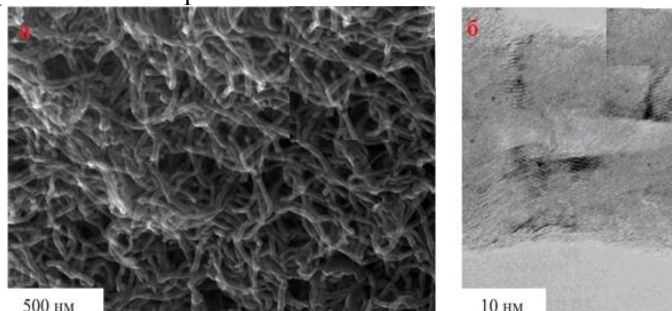
Figure-5. SEM and TEM images of MPC: a) and b) respectively.
