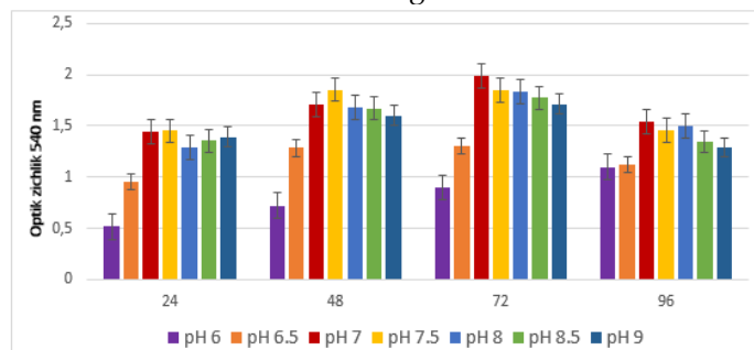
3-rasm. Hansschlegelia sp. - Shk-N2 shtamming o'sishiga ozuqa muhiti pH ko'rsatkichining ta'siri.
