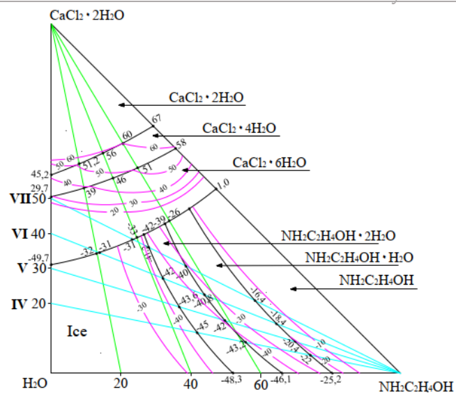
Fig. 2. Polythermal solubility diagram of the \text{CaCl}_2 \cdot 2\text{H}_2\text{O} - \text{NH}_2\text{C}_2\text{H}_4\text{OH} - \text{H}_2\text{O} system
