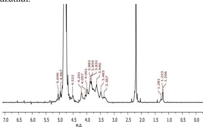
2-rasm. Ganoderma lucidum zamburug'idan ajratib olingan suvda eruvchan polisaxaridning ^1\text{H} YaMR spektri
